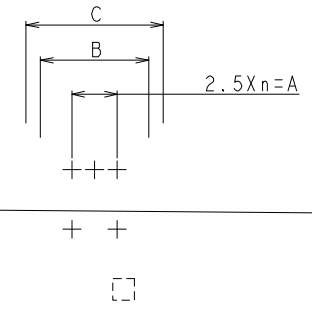
4POS(X-KEY):
