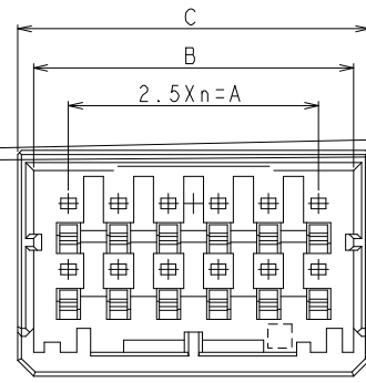
12POS(X-KEY):
